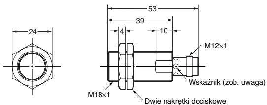
E2A-M18KS08-M1-□□/E2A-S18KS08-M1-□
