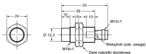
E2A-M18KN16-M1-□□/E2A-S18KN16-M1-□
