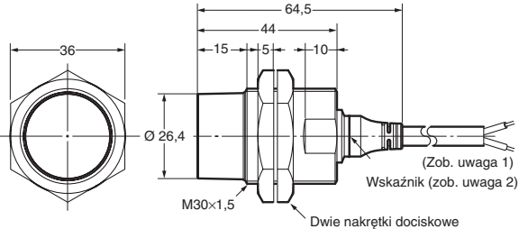
E2A-M30KN20-WP-□□/E2A-S30KN20-WP-□
