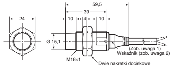
E2A-M18KN16-WP-□□/E2A-S18KN16-WP-□
